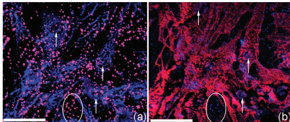
Figure 13. SIMS maps of fibroblast cells dosed with 50 ppm of dissolved Cr(III) and incubated for 7 h: (a) positive SIMS maps (blue \text{Ca}^+ , red \text{Cr}^+ ); (b) negative SIMS maps (red CN, blue \text{PO}_2 ). Scale bar = 50 \mu\text{m} . Reprinted with permission from ref 636. Copyright 2006 Elsevier.
